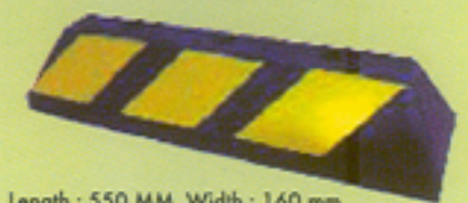
Length : 550 MM, Width : 160 mm Height 110 mm Weight 6 kg
